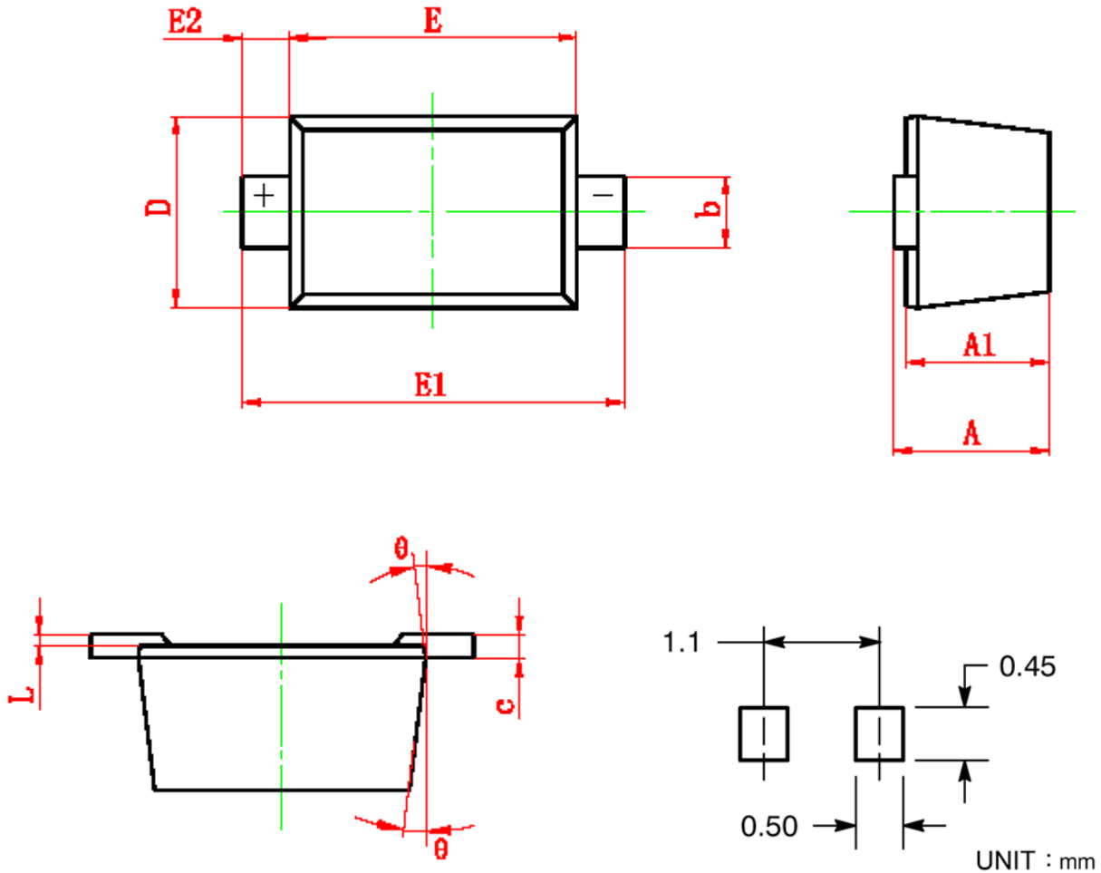
PCB Layout
